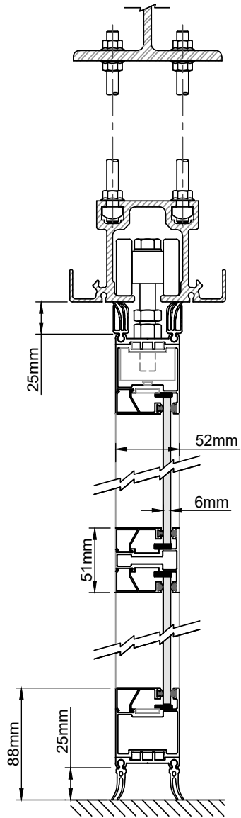
6MM GLASS
