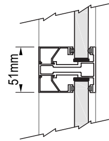
HORIZONTAL MULLION
