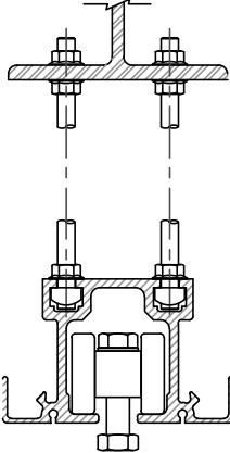
STEEL BEAM
